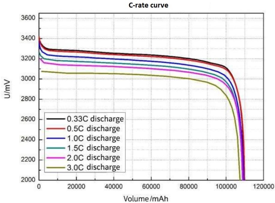
Graph 1: C-rate curve
