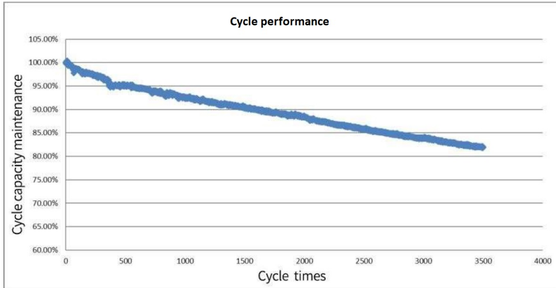
Graph 3: Cycle performance (1,0C) curve
